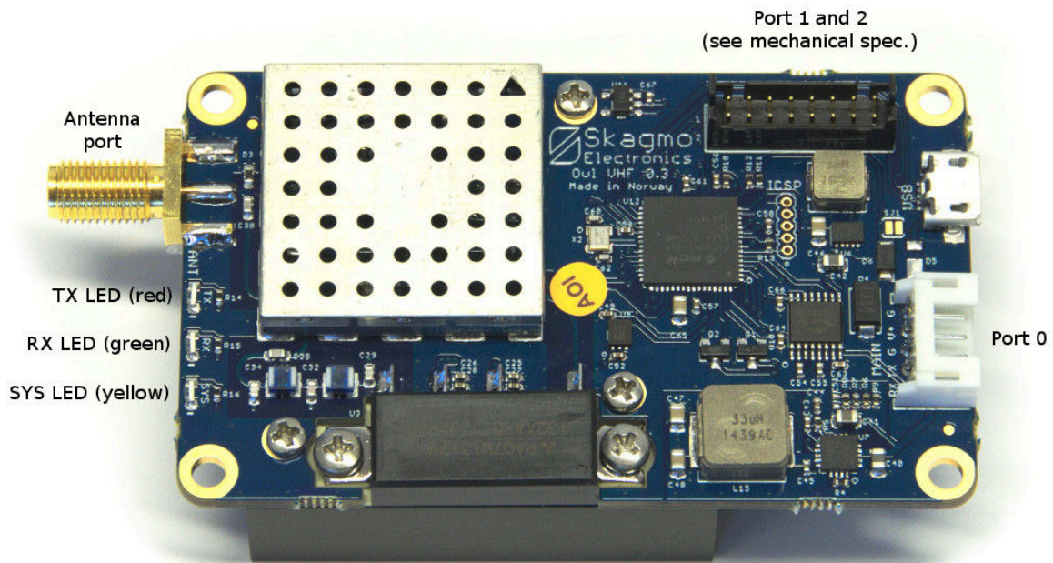
Figure 1: Board layout
